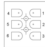
Plug view of screw terminals
